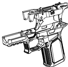
MODULAR PISTOL
